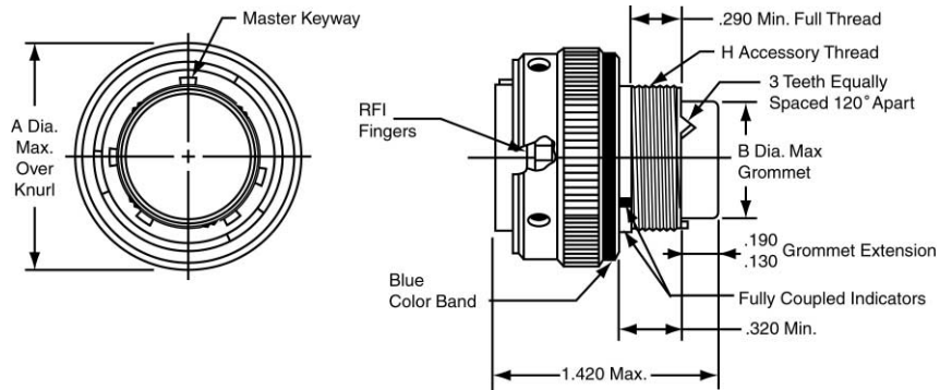
Plug Shell, RFI Grounding, Bayonet Coupling Military No. MS3475 Amphenol/Matrix No. MB18
