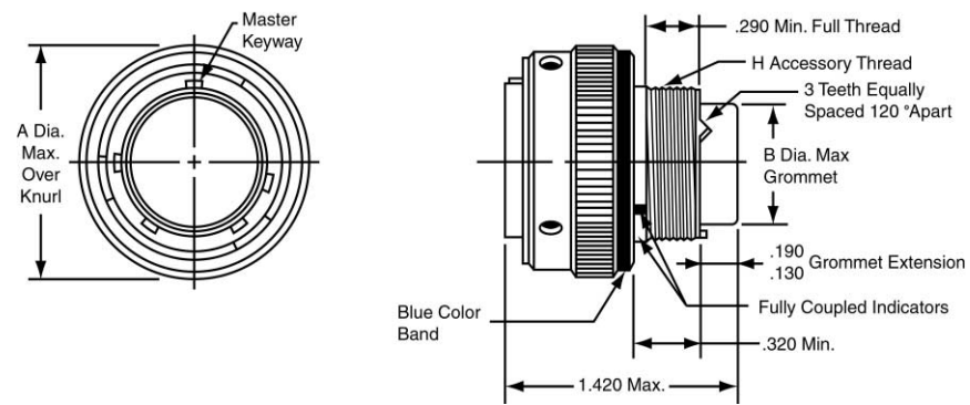
Plug Shell, Bayonet Coupling Military No. MS3476 Amphenol/Matrix No. MB16
