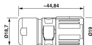
Dimensioned drawing
