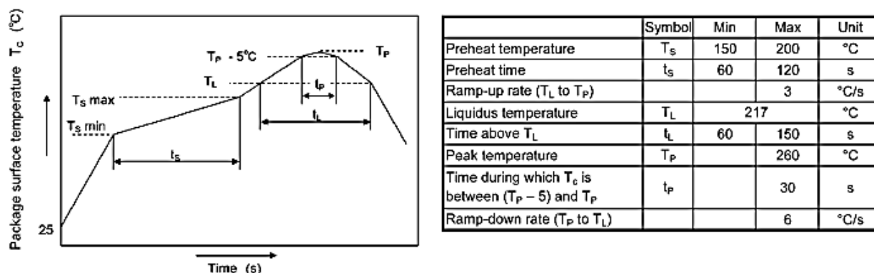
Fig. An example of a temperature profile when lead(Pb)-free solder is used
