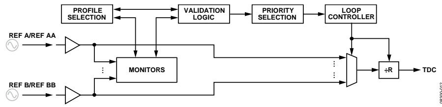
Figure 36. Reference Clock Block Diagram
