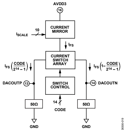
Figure 43. DAC Output Pins
