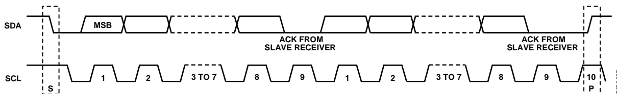
Figure 62. Acknowledge Bit
