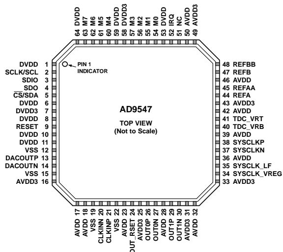
Figure 2. Pin Configuration
