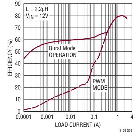
Efficiency, V_{OUT} = 1.8V , f_{SW} = 2\text{MHz}
