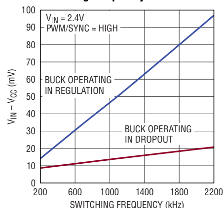
V_{CC} LDO Voltage Drop vs Switching Frequency
