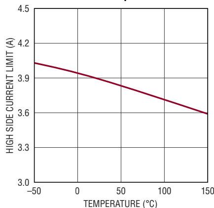
High Side Current Limit Threshold vs Temperature
