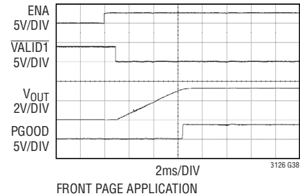
Start-Up Waveforms
