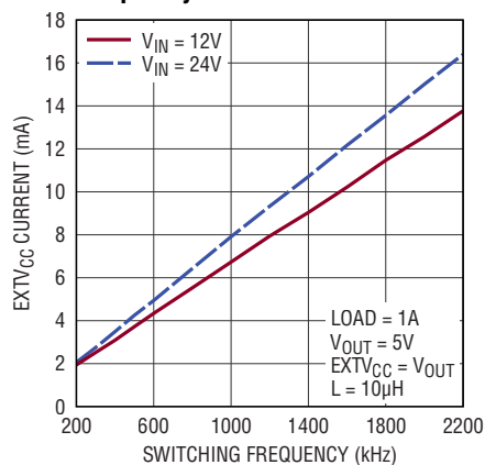
\text{EXTV}_{CC} Current vs Switching Frequency
