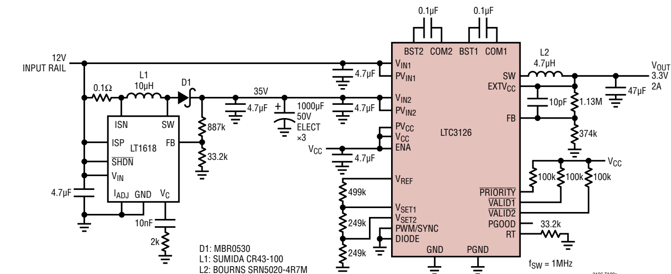
V_{OUT} Hold-Up with Loss of Input Supply
