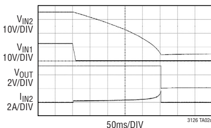
V_{OUT} Hold-Up with Loss of Input Supply
