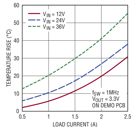
Temperature Rise vs Load Current
