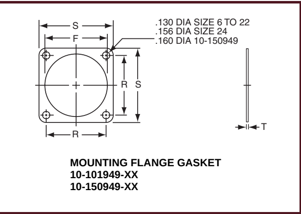
MOUNTING FLANGE GASKETS – FOR PT, SP, PC
