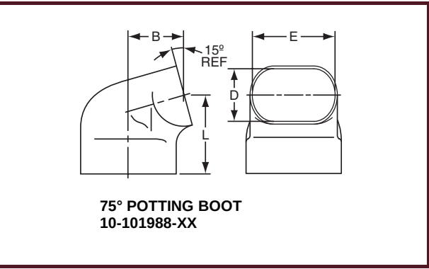
75° POTTING BOOTS – FOR PT, SP, PC
