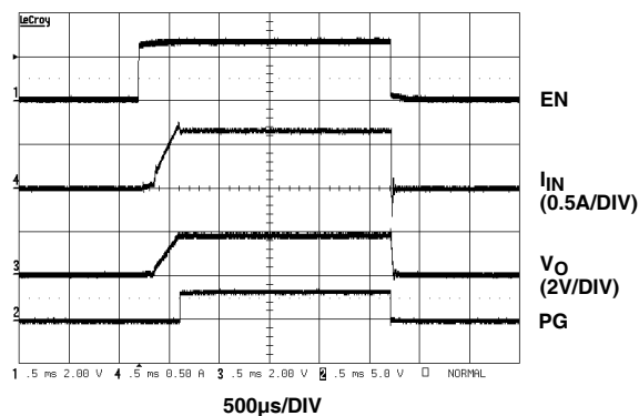
FIGURE 14. ENABLE AND SHUT-DOWN
