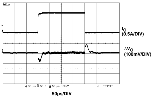
FIGURE 20. PWM LOAD TRANSIENT RESPONSE (0A TO 1A)
