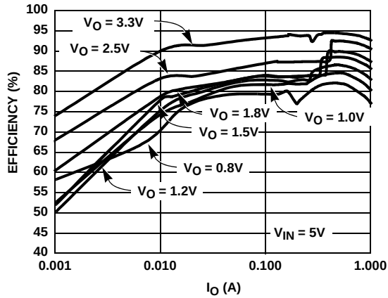
FIGURE 1. EFFICIENCY vs I_O (PFM/PWM MODE)
