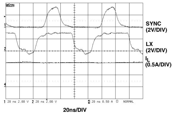
FIGURE 18. EXTERNAL SYNCHRONIZATION TO 12MHz
