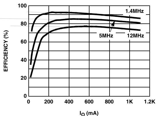
FIGURE 10. EFFICIENCY vs I_O (PWM MODE)
