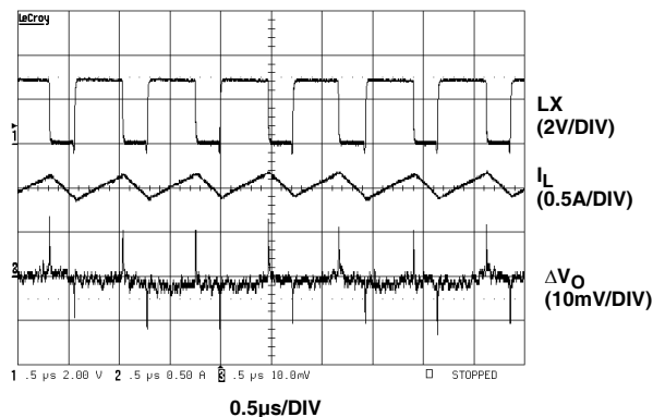
FIGURE 16. PWM STEADY-STATE OPERATION ( I_O = 1A )
