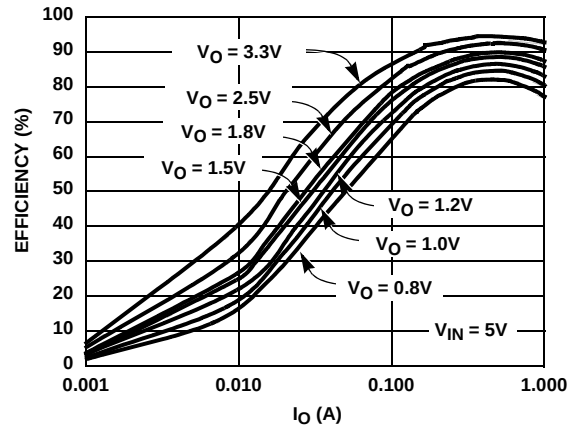
FIGURE 2. EFFICIENCY vs I_O (PWM MODE)
