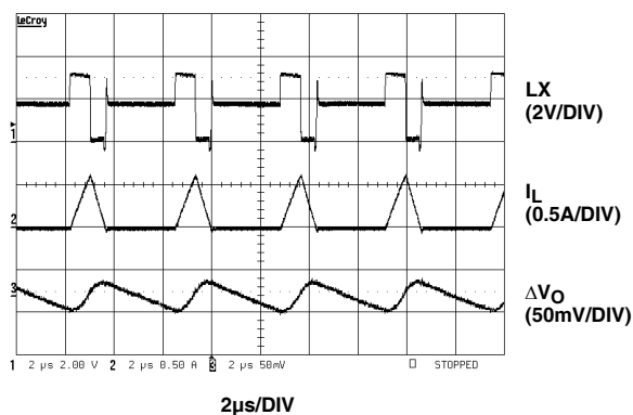
FIGURE 15. PFM STEADY-STATE OPERATION WAVEFORM ( I_O = 100mA )
