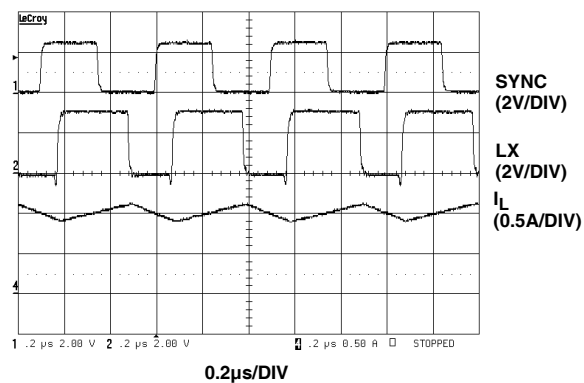
FIGURE 17. EXTERNAL SYNCHRONIZATION TO 2MHz
