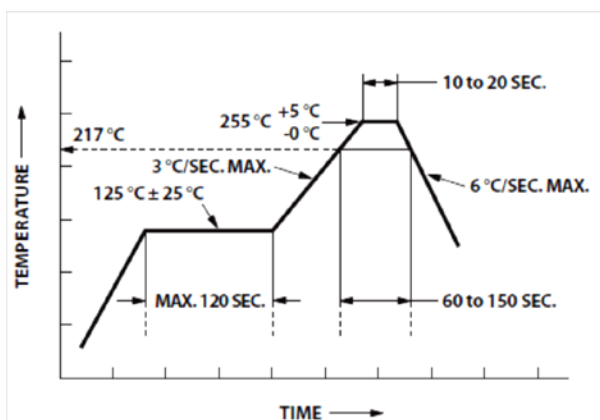
Figure 6. Recommended Pb-free reflow soldering profile.
