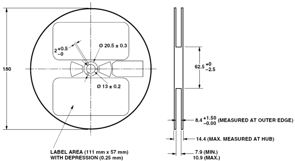
Figure 12. Reel dimensions.
