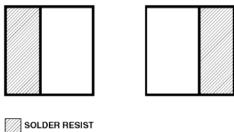
Figure 8. Recommended soldering pad pattern.
