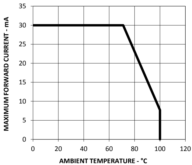
Figure 4. Maximum forward current vs. ambient temperature. Derated based on T_{J\text{ MAX}} = 110^{\circ}\text{C} , R_{\theta\text{ JA}} = 500^{\circ}\text{C/W} .
