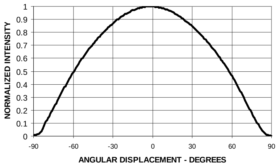
Figure 5. Radiation Pattern.
