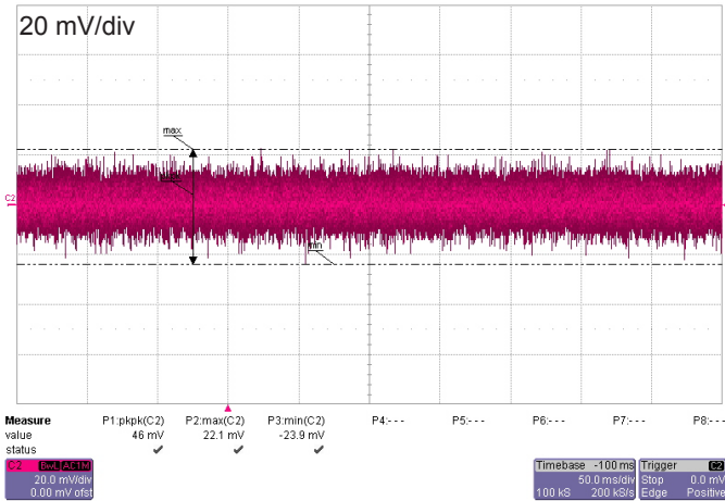
Figure 10: Output noise
