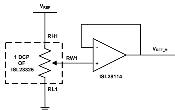
FIGURE 2. V_{\text{REF}} ADJUSTMENT
