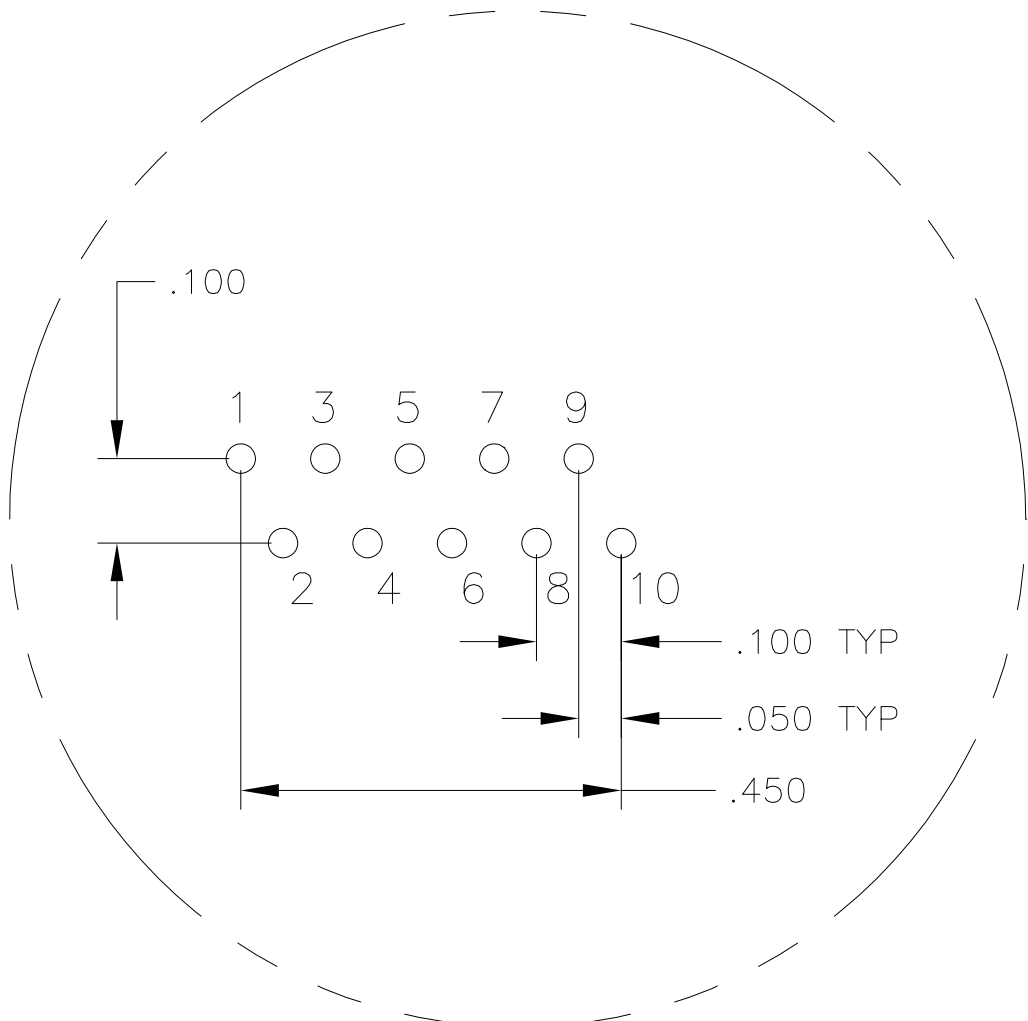
Pin Designations
