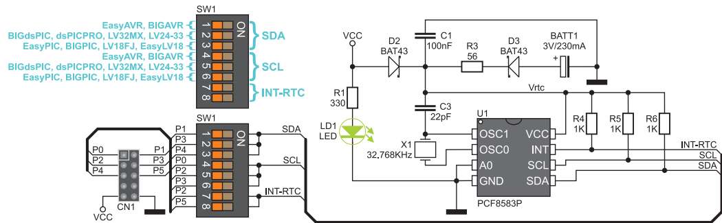
Figure 3: RTC board connection schematic
