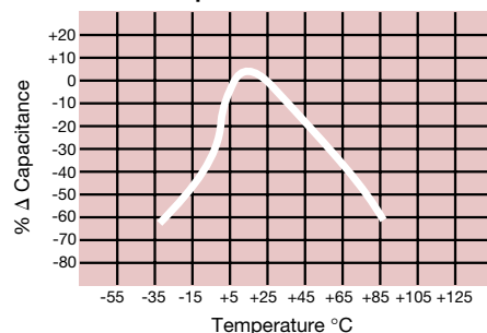
Temperature Coefficient
